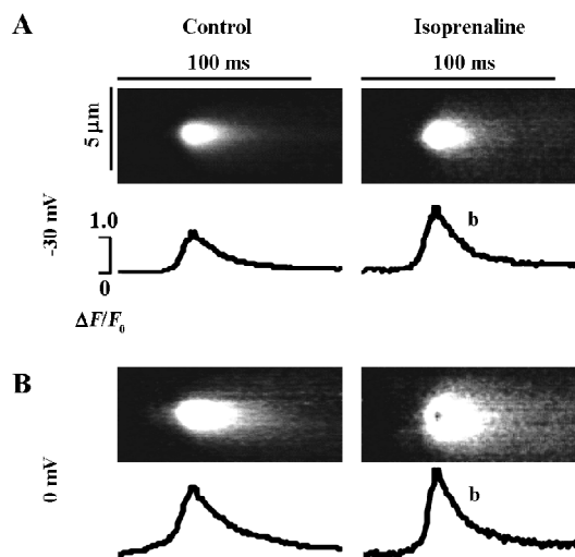
Figure 3. Effect of isoprenaline on averaged sparks at different voltages. (A) Averaged spark at \sim 30 mV. From top to bottom: averaged line-scan images of sparks at peak, time courses of the corresponding line-scan images (spatially averaged over 1.1- \mu m width); left: averaged spark under the control condition; right: averaged spark after isoprenaline ( 1 \mu\text{mol}\cdot\text{L}^{-1} ) treatment. (B) Averaged spark at \sim 0 mV. b P < 0.05 vs control.
